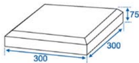
300x300x75 Type - D
