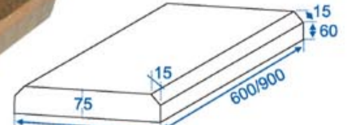
600 or 900x300x75 Type - E
